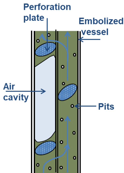
Movement of water in xylem vessels
