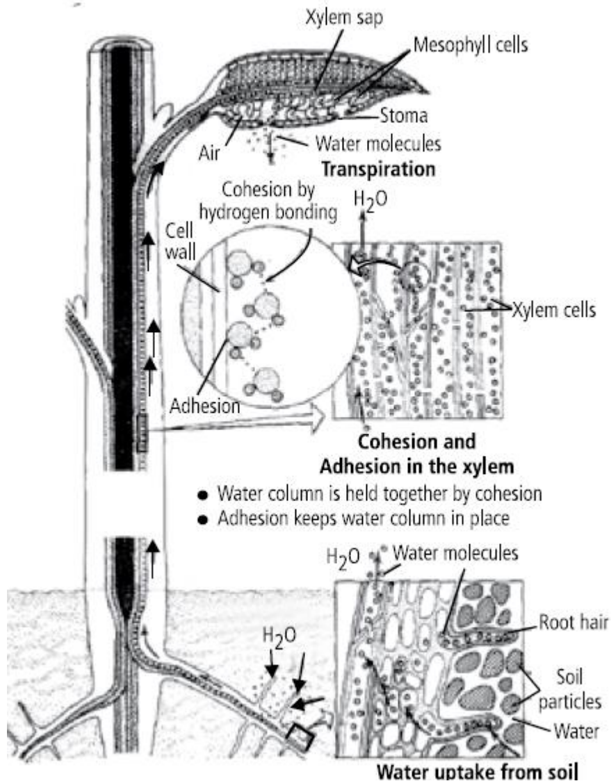
Diagram of "Ascent of sap" author by unknown source retrieved from https://www.google.com/search?q=ascent+of+sap+in+plants&sxsrf=ALeKk01QSAf2M7S1gCPzD4XTrUK8P3rH5A:1607758083478&source=lnms&tbm=isch&sa=X&ved=2ahUKEwjJ3czL9cftAhXBzDgGHRzeBaIQ_AUoAXoECBwQAw&biw=1536&bih=754#imgsrc=WEH1bCRIHZqV0M under free repository
